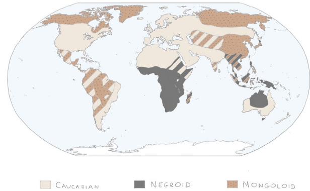
Figure. Simplified distribution of races around the world.
